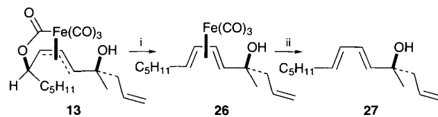
Scheme 3 Reagents and conditions: i, \text{Ba}(\text{OH})_2 (saturated aqueous solution), MeOH, 20 min, 85%; ii, \text{H}_2\text{O}_2 , NaOH, MeOH, 0^\circ\text{C} , 25 min, 72%
